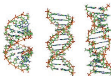
ADN
