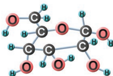
Glucosa
